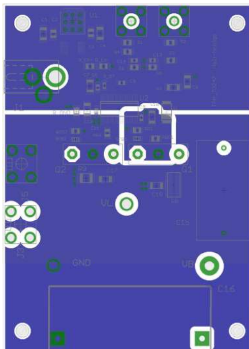
Half-bridge layout Sample (Bottom Layer)
